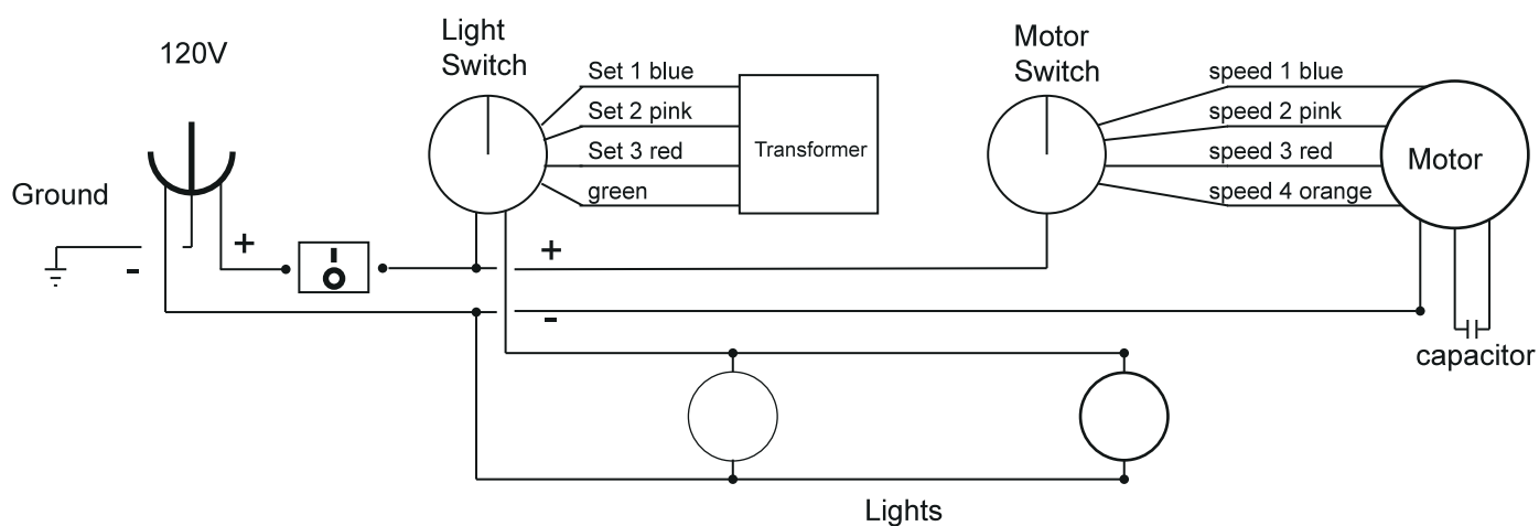
Wiring Diagram
